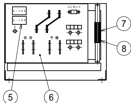
裏面端子盤
